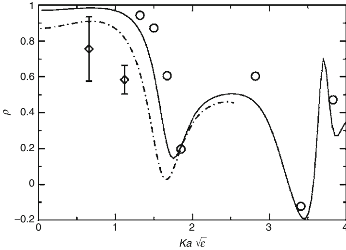
Fig. 17.3 Polarization anisotropy ratio as a function of reduced optical radius ka\sqrt{\epsilon} , where \epsilon is the dielectric constant of the material. Solid (broken) lines are the theoretical curves for Si (SiC) NWs. Circles (diamonds) are the experimental values for Si (SiC) NW optical phonon (TO) lines (With permission from reference [12]. Copyright (2006) by the American Physical Society)
