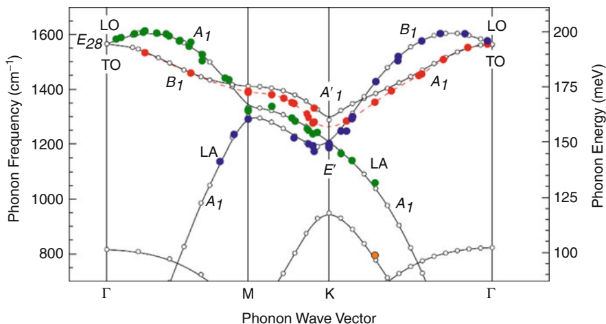
Fig. 7.4 Phonon dispersion of graphite from inelastic X-ray scattering along the in-plane high symmetry directions ( full circles ). The dashed line is a cubic-spline interpolation to the TO-derived branch. The open circles show an ab-initio calculation for graphene, downscaled by 1% (Reprinted with permission from Maultzsch J, Reich S, Thomsen C, Requardt H, Ordejón P (2004) Phonon dispersion in graphite. Physical Review Letters 92 (7): 075501-1-4. Copyright (2004) by the American Physical Society)
