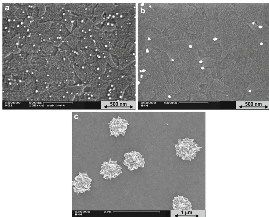
Fig. 8.7 SEM images of isolated gold clusters electrodeposited on ITO covered glass [37]. (a) Single pulse ( E_1 = -100 mV/ = 0.1 s), (b) double-pulse ( E_1 = -100 mV/0.1 s; E_2 = +800 mV/ 90 s), (c) double-pulse ( E_1 = -100 mV/0.1 s; E_2 = +600 mV/90s)
