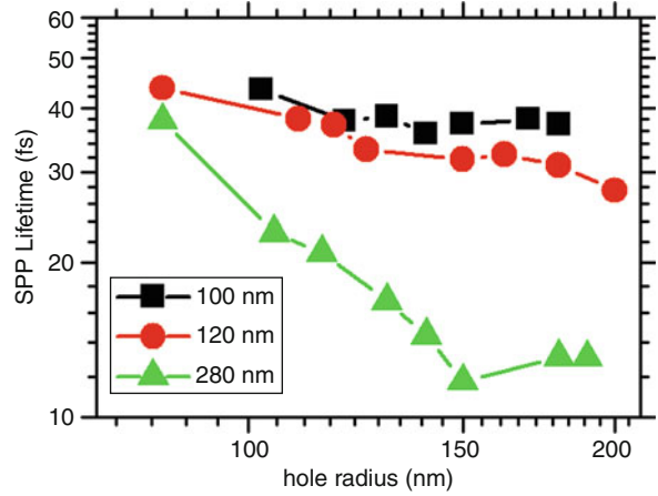
Fig. 1.18 The dependence of \tau_{\text{SPP}} on hole radius for different depths taken at \lambda_{\text{res}} = 800 nm
