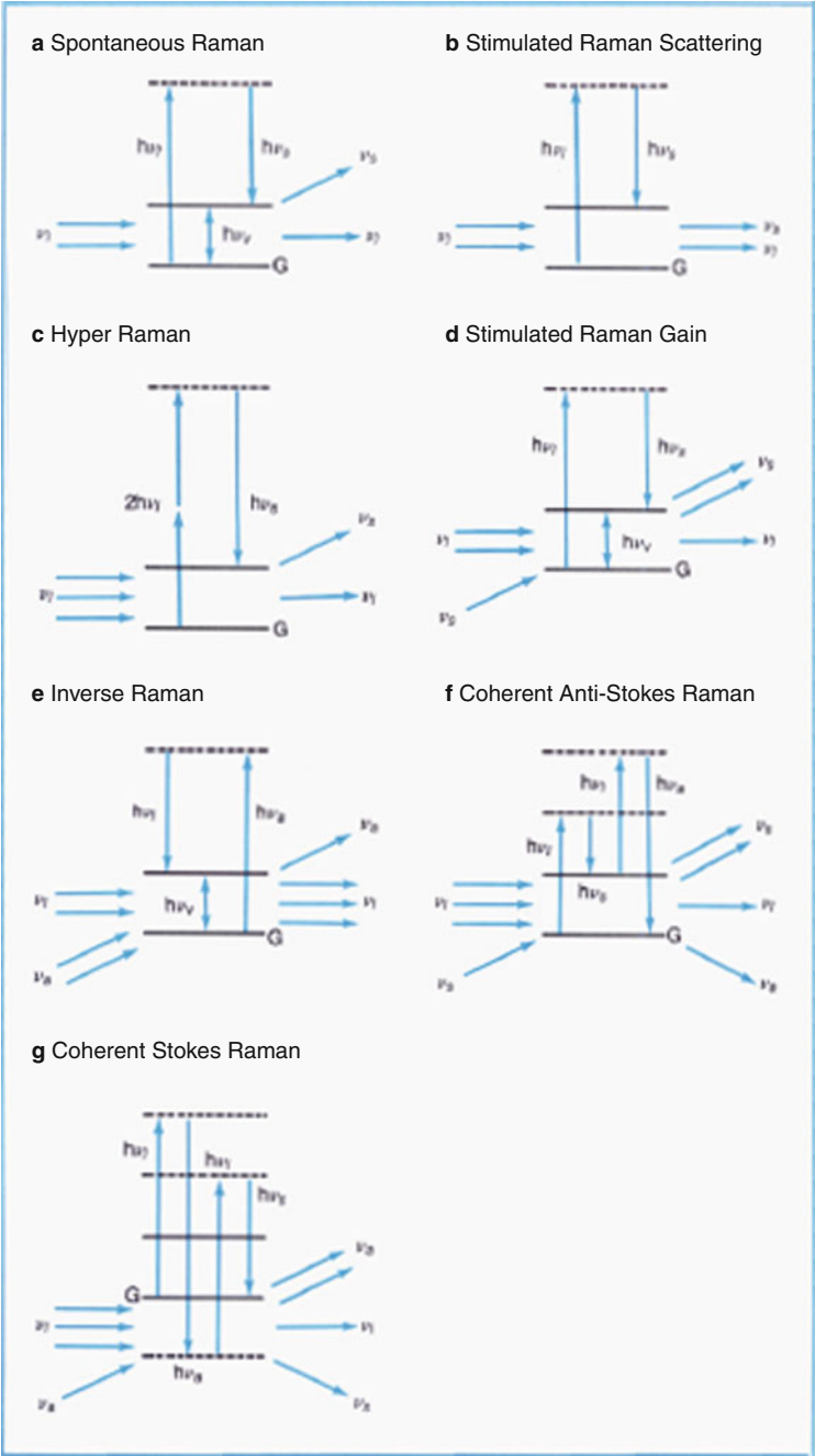
Fig. 3 Quantum diagrams of different nonlinear Raman processes [10]
