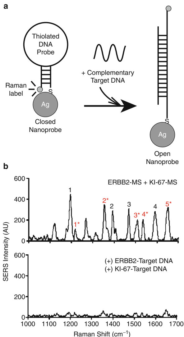
Fig. 13.7 The operating principle of the SERS-based molecular sentinel (MS) nanoprobe. (a) The MS nanoprobe is composed of a Raman-labeled DNA hairpin probe and a silver nanoparticle. In the absence of the complementary target DNA, a strong SERS signal is observed due to the hairpin conformation adopted by the MS nanoprobe ( left: closed state ). (b) In the presence of the complementary target DNA, the hairpin conformation of the MS nanoprobe is disrupted and the SERS signal is quenched due to the physical separation of the Raman label from the surface of the silver
