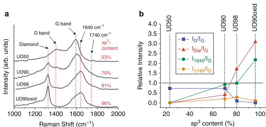
Fig. 12.13 (a) Raman spectra of different ND powders with \text{sp}^3 contents ranging from 23% to 96%. (b) Changes in the intensity of D band, diamond peak, and Raman features at 1,640 and 1,740 \text{cm}^{-1} . Intensities were normalized to the G band intensity at 1,590 \text{cm}^{-1}
