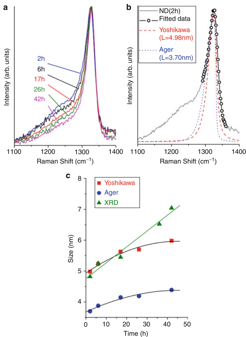
Fig. 12.20 (a) Diamond Raman peak recorded after oxidation at 430^{\circ}\text{C} for 2, 6, 17, 26, and 42 h in air. (b) Raman spectrum of ND powder oxidized for 2 h at 430^{\circ}\text{C} in air and corresponding peak fit. Data used for peak fitting is indicated by the circles . (c) Calculated crystal size for ND powders oxidized for 2, 6, 17, 26, and 42 h at 430^{\circ}\text{C} . X-ray diffraction data is shown for comparison
