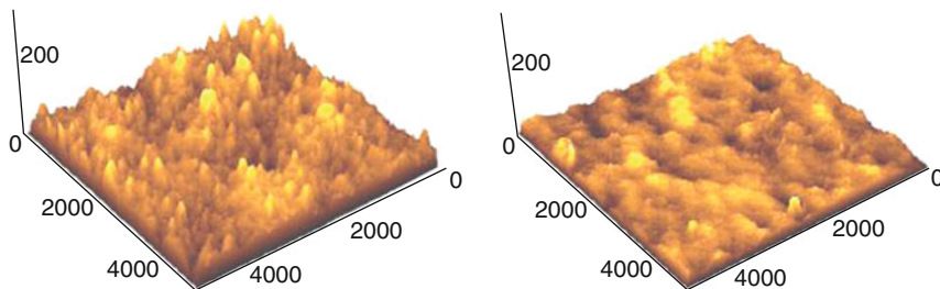
Fig. 20.13 AFM images of alumina filters coated with Ag particles with ( left ) and without ( right ) chloride anions
