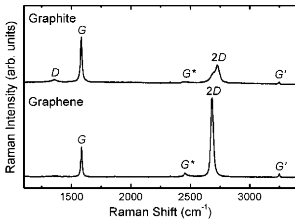
Fig. 9.6 Raman spectra of graphene and graphite
