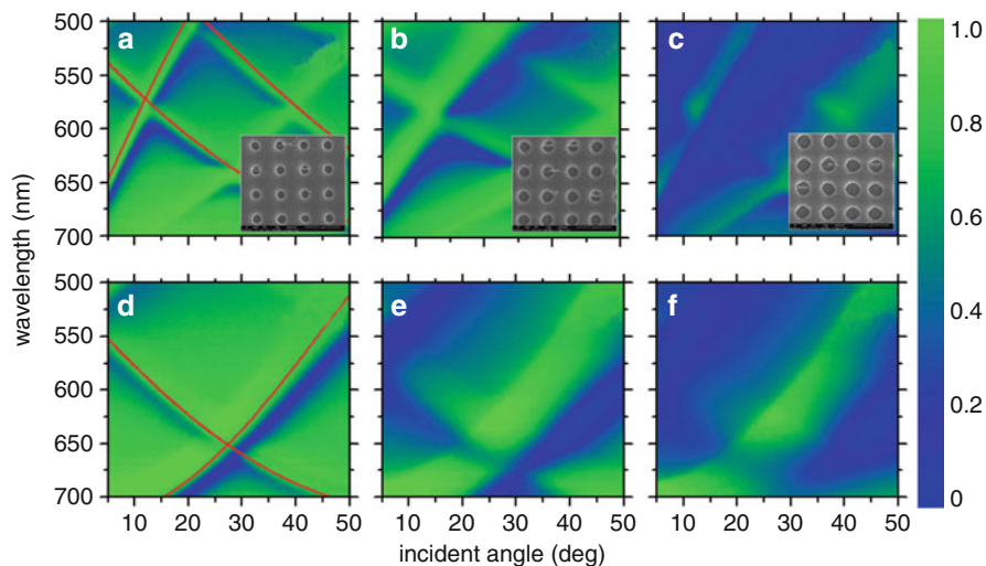
Fig. 1.15 The (a–c) p-p and (d–f) s-s reflectivity mappings of 2D Ag circular hole arrays with hole radius = 85, 140, and 180 nm (from left to right ) and depth = 280 nm. The dash lines are deduced from the SPP phase-matching equation indicating (1,0), (−2,0), and (−1,±1) s SPPs are excited under p-polarization while (0,±1) a and (−1,±1) a SPPs are excited under s-polarization. The corresponding SEM images are shown in the insets. At larger hole radius, localized resonance evolves and actually couple with the SPPs making the features become blurry
