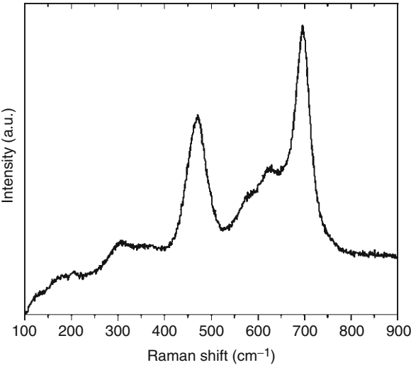
Fig. 14.5 Raman spectra of an as-grown CoFe 2 O 4 single crystal measured at room temperature (Reprinted with permission from Ref. [40]. Copyright Elsevier B.V. (2006))
