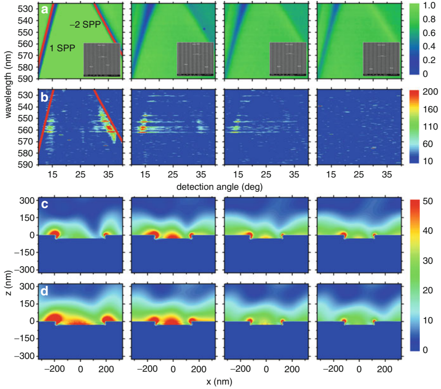
Fig. 1.11 The (a) p-p reflectivity mapping of Ag gratings with period = 650 nm, depth = 30 nm and groove width = 377, 277, 247, and 230 nm (from left to right). The dash lines are deduced from the SPP phase-matching equation revealing 1 and -2 SPPs are excited. Insets are the corresponding SEM images. (b) The p-p Raman detection mappings of the same gratings taken at incident angle = \sim 20^\circ . RCWA simulations of electric field intensity at (c) 514 nm, \sim 20^\circ and (d) 562 nm, \sim 13^\circ
