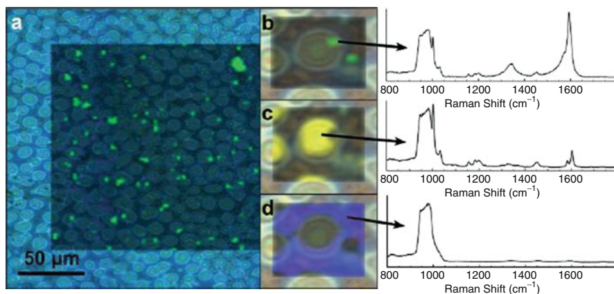
Fig. 15.3 (a) Raman map of PS-functionalized SWCNT highlighted in green. Insets indicate the signal from the three components: SWCNT (b), PS (c), PMMA (d). The corresponding Raman spectra are shown on the right (Reprinted from [12])
