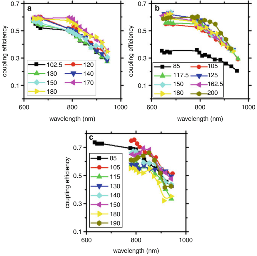
Fig. 1.19 The plots of coupling efficiency of (1,0) and (−1,0) SPP modes with resonant wavelength \lambda_{\text{res}} at different hole radii and depths = (a) 100 nm, (b) 120 nm, and (c) 280 nm. The legends are hole radius in the unit of nm
