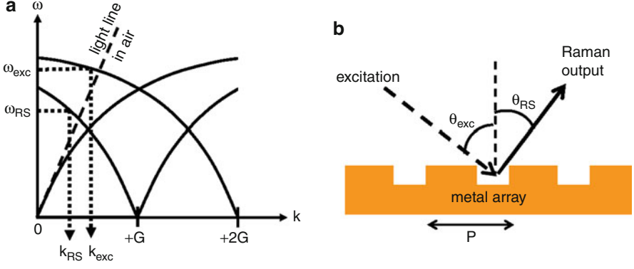
Fig. 1.2 (a) The (partial) dispersion relation of SPPs on 1D metallic array with period P (solid lines). Part of the dispersion relation now is within the light line (dash line) and excitation of ingoing and outgoing SPPs is possible if the laser and Raman emission at \omega_{exc} and \omega_{RS} follow the dispersion relation at k_{exc} and k_{RS} (dot lines). (b) Strong Raman intensity is observed from the array when the laser and the Raman emission are impinged at and collected from the array at \theta_{exc} and \theta_{RS} given as k = \frac{\omega}{c} \sin \theta \pm n \frac{2\pi}{P}
