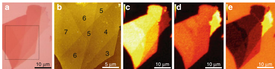
Fig. 9.14 (a) Optical microscope image and (b) AFM (contact mode) image of a graphene sample. Images of (c) the G band intensity, (d) the 2D band intensity, and (e) the ratio of the intensity of the 2D band to that of the G band [24]
