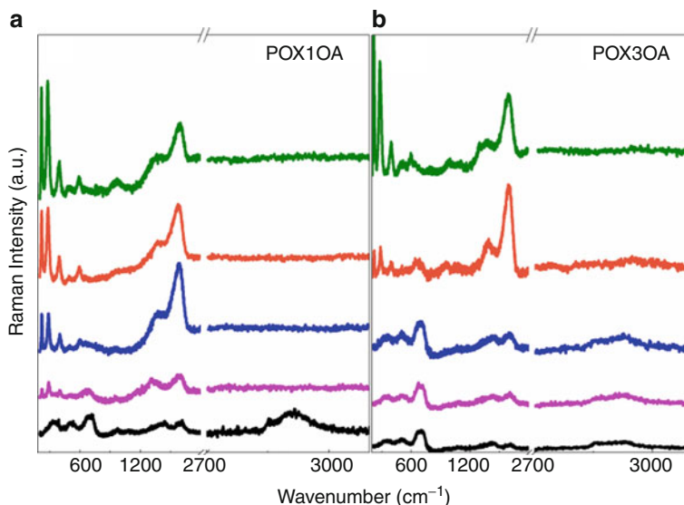
Fig. 14.15 Room-temperature Raman spectra of samples (a) POX1OA and (b) POX3OA, under the laser excitation intensity of 0.5, 1.6, 3.2, 6.4, and 16.1 mW (from bottom to top ) (Reprinted with permission from Ref. [55]. Copyright American Chemical Society (2010))
