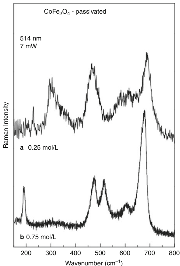
Fig. 14.12 Raman spectra of \text{CoFe}_2\text{O}_4 samples (a) peptized at 0.25 mol/L perchloric acid) and (b) peptized at 0.75 mol/L perchloric acid. Reprinted with permission from Ref. [50]. Copyright Elsevier B.V. (2004)
