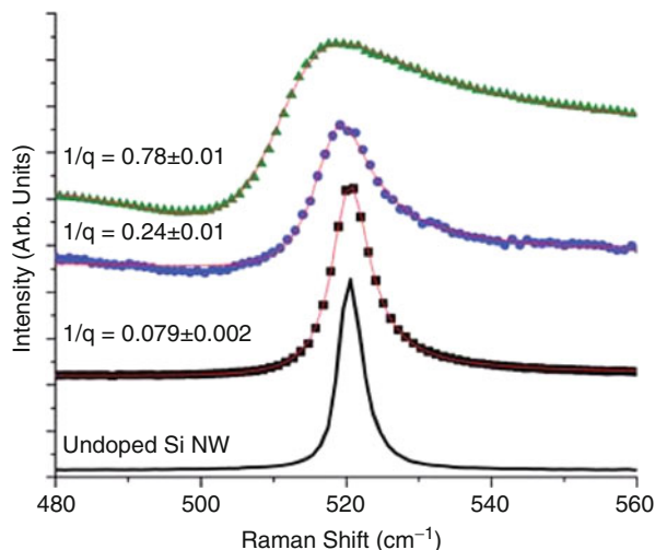
Fig. 17.8 Raman spectra from individual Si NWs (excitation wavelength of 633 nm) with different active boron concentrations. Fano fitting renders 1/q values of (bottom to top) \sim 0.079 , \sim 0.24 , and \sim 0.78 , corresponding respectively to approximate active boron concentrations of \sim 1\text{--}2 \times 10^{19} , \sim 5 \times 10^{19} , and greater than 1 \times 10^{20} \text{ cm}^{-3} (Adapted with permission from reference [47]. Reproduced by permission of the Royal Society of Chemistry ( http://dx.doi.org/10.1039/C0NR00127A ))
