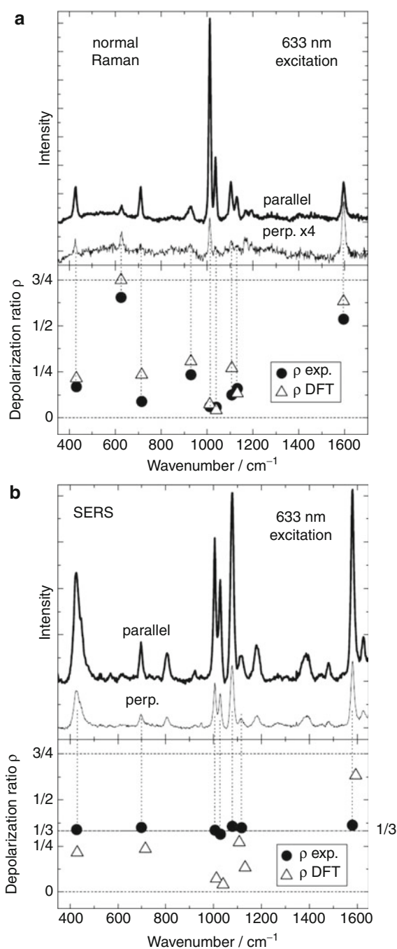
Fig. 10.8 Polarized Raman spectra and depolarization ratios of benzenethiol under (a) normal Raman and (b) SERS conditions.
