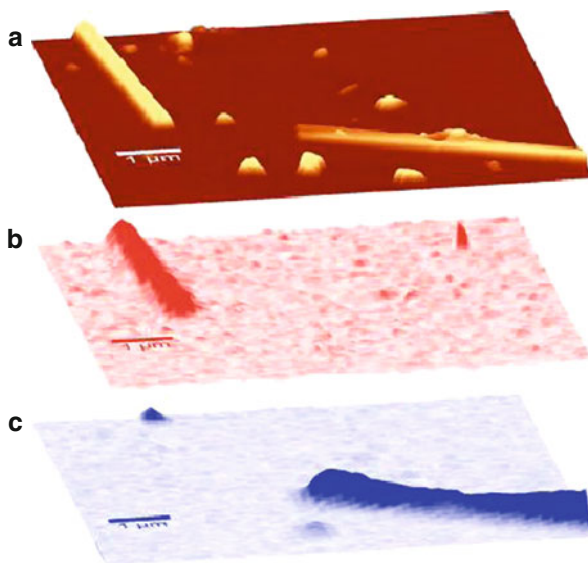
Fig. 15.4 (a) AFM topographic images of VO 2 and V 2 O 5 nanowires. (b) Map of integrated Raman signal (615–625 cm -1 ) in the same region identifying VO 2 nanowire. (c) Map of integrated Raman signal (989–999 cm -1 ) identifying V 2 O 5 nanowire (Reprinted from [13])
