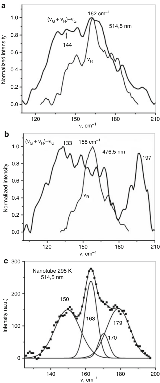
Fig. 7.12 Comparison of normalized bands of low-frequency mode and sum tone \nu_G + \nu_{RBM} under excitation with \lambda_L = 514.5 (a) and 476.5 nm (b); decomposition of low-frequency “breathing” mode of SWCNT \nu_{RBM} to individual components (c)
