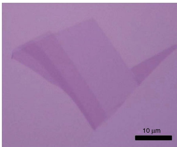
Fig. 9.1 Optical microscope image of graphene on \text{SiO}_2/\text{Si} . The lightest-colored area corresponds to single-layer graphene
