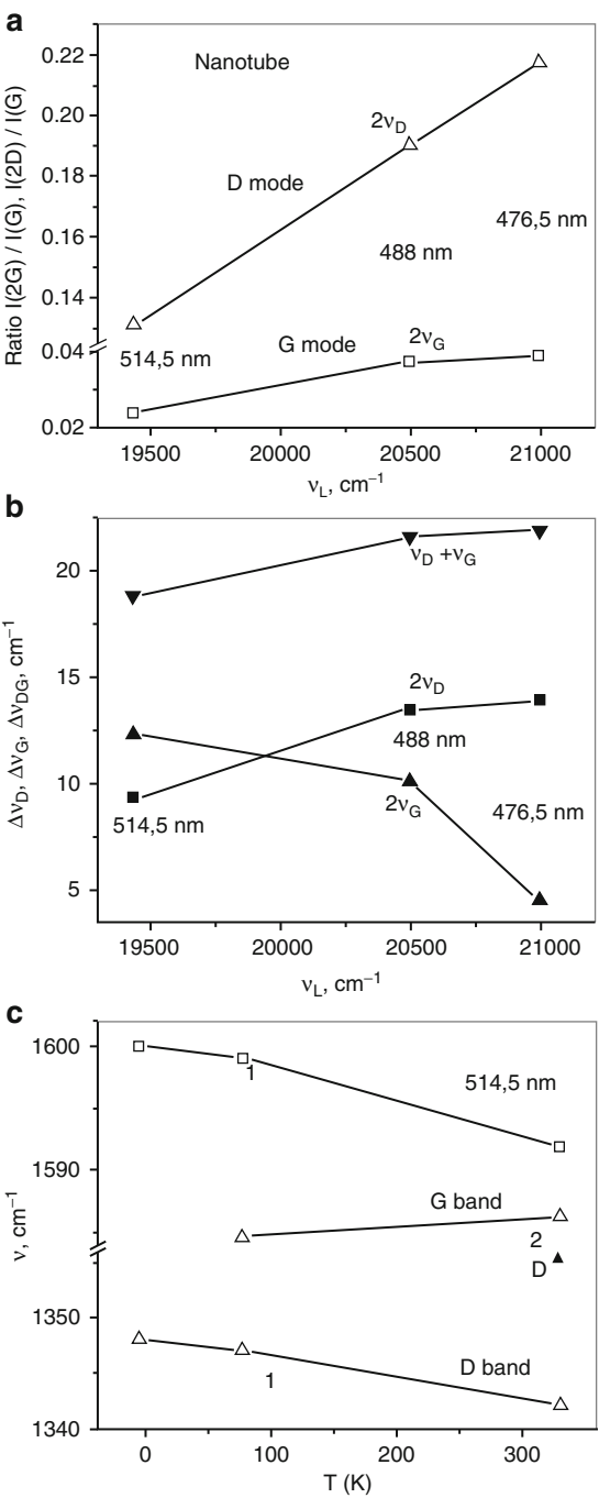
Fig. 7.11 Dependence of the ratios of the second-order to the first-order Raman band intensities (a) and of the experimentally observed harmonic bands (b) on the excitation frequency \nu_L (b) . (c) Temperature dependencies of the G and D Raman bands of SWCNTs (1) and graphite crystals (2)
