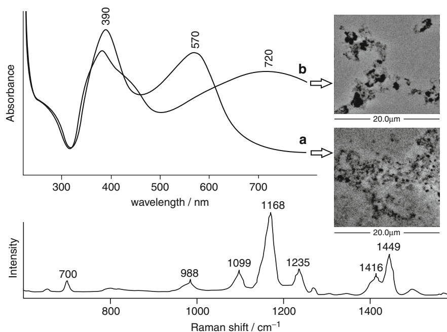
Fig. 20.12 Extinction spectra of Ag colloids with (b) and without (a) chloride anions, with the corresponding SEM images. In the lower panel, the SERS of 1H-1,2,3-triazole is shown. Exciting line: 514.5 nm
