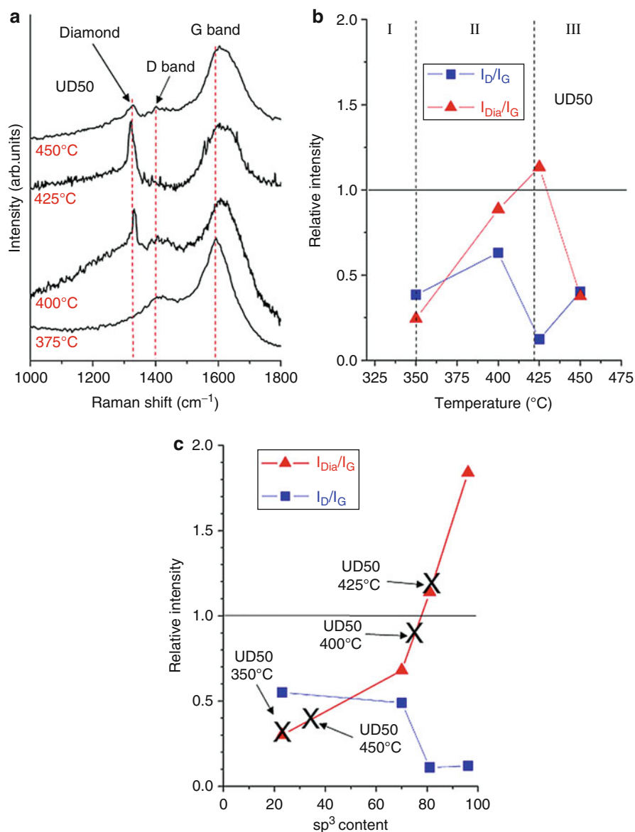
Fig. 12.15 (a) UV (325 nm) Raman spectra of UD50 after oxidation for 5 h at 375°C, 400°C, 425°C, and 450°C in air. (b) Relative intensity of diamond peak ( I_{\text{Dia}}/I_{\text{G}} ) and D band ( I_{\text{D}}/I_{\text{G}} ) in the after oxidation of UD50 normalized with respect to the G band intensity at 1,590 \text{cm}^{-1} . (c) Diamond content of oxidized UD50 (black cross) estimated using the relationship between I_{\text{Dia}}/I_{\text{G}} and the \text{sp}^3 content as determined by XANES for different ND samples (red triangles)
