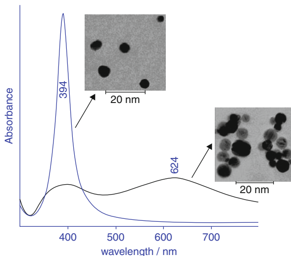
Fig. 20.4 Extinction spectra of pure Ag and adenine/Ag colloids with the corresponding TEM images
