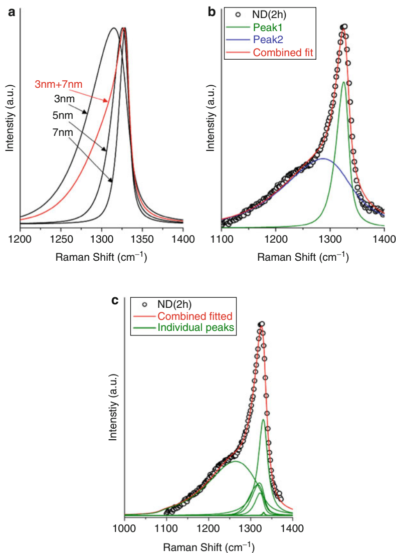
Fig. 12.21 (a) Calculated Raman spectra for different ND crystal sizes (black) in comparison to that of a sample containing a binary size-distribution (red). (b) Raman spectrum of oxidized ND (2 h at 430°C) fitted using two peaks to account for contributions from both small and large crystals as well as lattice defects. (c) Raman spectrum of oxidized ND (2 h at 430°C) fitted using seven peaks, each representing the contribution of a different dispersion relation
