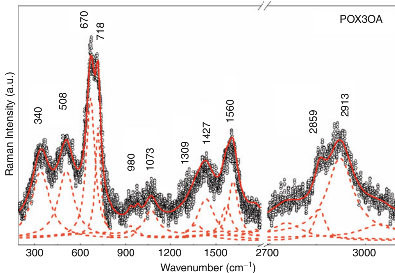
Fig. 14.14 Room-temperature Raman spectrum of POX3OA (Reprinted with permission from Ref. [55]. Copyright American Chemical Society (2010))
