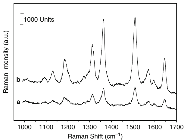
Fig. 6.6 Raman spectra obtained at the surfaces of Ag-coated ITO (a) and Ag-MWCNTs-ACS-coated ITO for 10^{-4} M R6G in aqueous solution (Reprinted with permission from Ref. [17]. © 2009 Elsevier)
