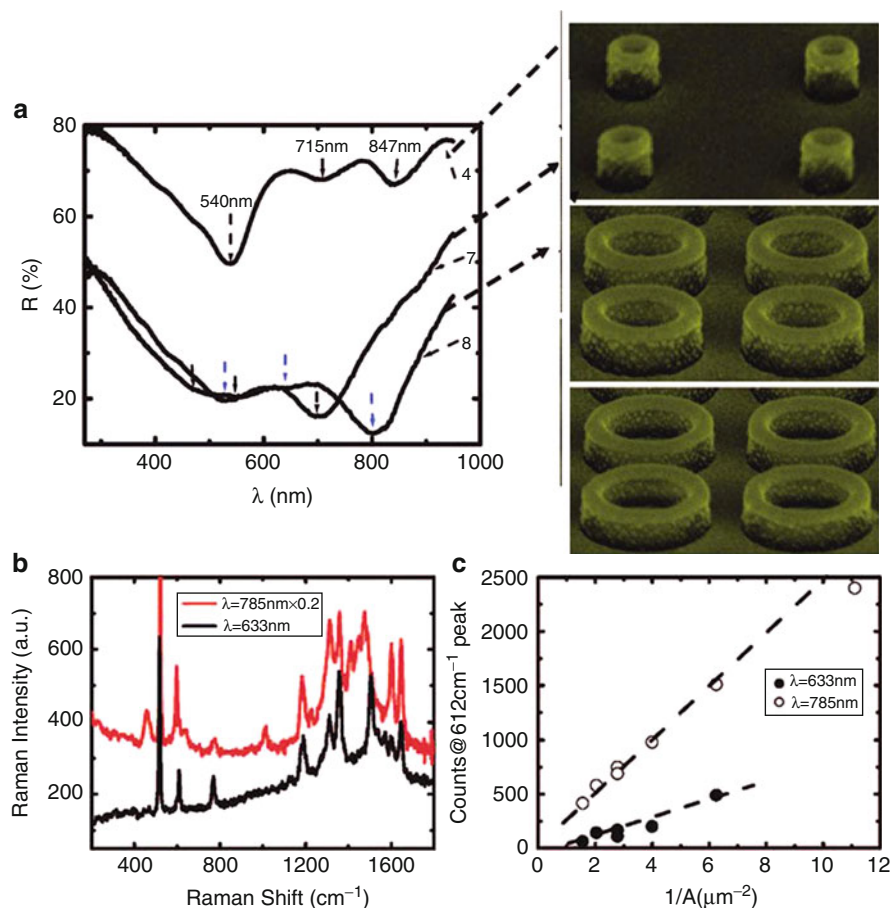
Fig. 10.14 (a) UV-vis spectra and SEMs of Au nanowells with different aspect ratios and pitches. (b) SERS spectra of Rh6G from Au nanowells and (c) intensity of the 612 cm -1 mode as a function of the number of nanowells per unit area (Figure reproduced from Ref. [175])
