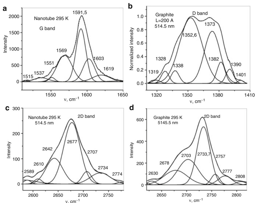
Fig. 7.10 Results of numerical deconvolution of the main bands and harmonic tones in Raman spectra into composing lines: \nu_G band of SWCNT (a), \nu_D band of an isotropic polycrystalline graphite (b), 2\nu_D tone spectrum of SWCNT (c), and 2\nu_D tone spectrum of the graphite single crystals (d)
