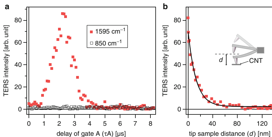
Fig. 16.15 (a) TERS intensity of carbon nanotubes measured while scanning one of two gates through the entire tapping oscillation (filled square: a vibrational frequency of the G-band at 1595\text{ cm}^{-1} ; open square: no vibrational frequency at 850\text{ cm}^{-1} ). (b) Distance dependence of TERS intensity of the G-band derived from (a). The delay time is converted to tip-sample distance by taking into account the harmonic oscillation of the tip (Reprinted from [66], Copyright 2007, with permission from American Institute of Physics)
