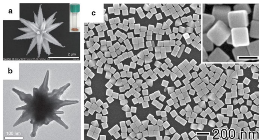
Fig. 10.13 (a, b) SEM images of gold mesoflowers produced by Sajanalal et al. (c) SEM images of silver nanocubes. Scale bar on the inset corresponds to 100 nm (Figure reproduced from Refs. [150] and [142])
