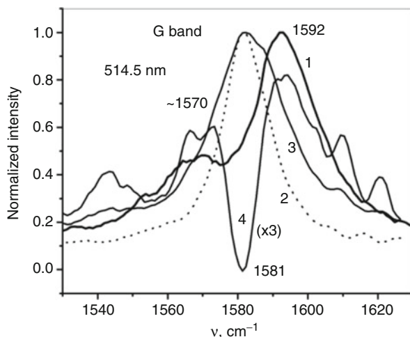
Fig. 7.7 Comparison of Raman spectra for carbon nanotubes (1) and normalized G-bands of a single crystalline (2) polycrystalline anisotropic graphite sample with oriented grains and L \approx 300 Å (3) and the difference spectrum corresponding to the curves 2 and 3 (4). All spectra correspond to room temperature and excitation with \lambda_L = 514.5 nm and are normalized to the maximum of the intensity of the corresponding Raman band. The difference spectrum (4) is multiplied by a factor of 3 for better comparison with the other spectra
